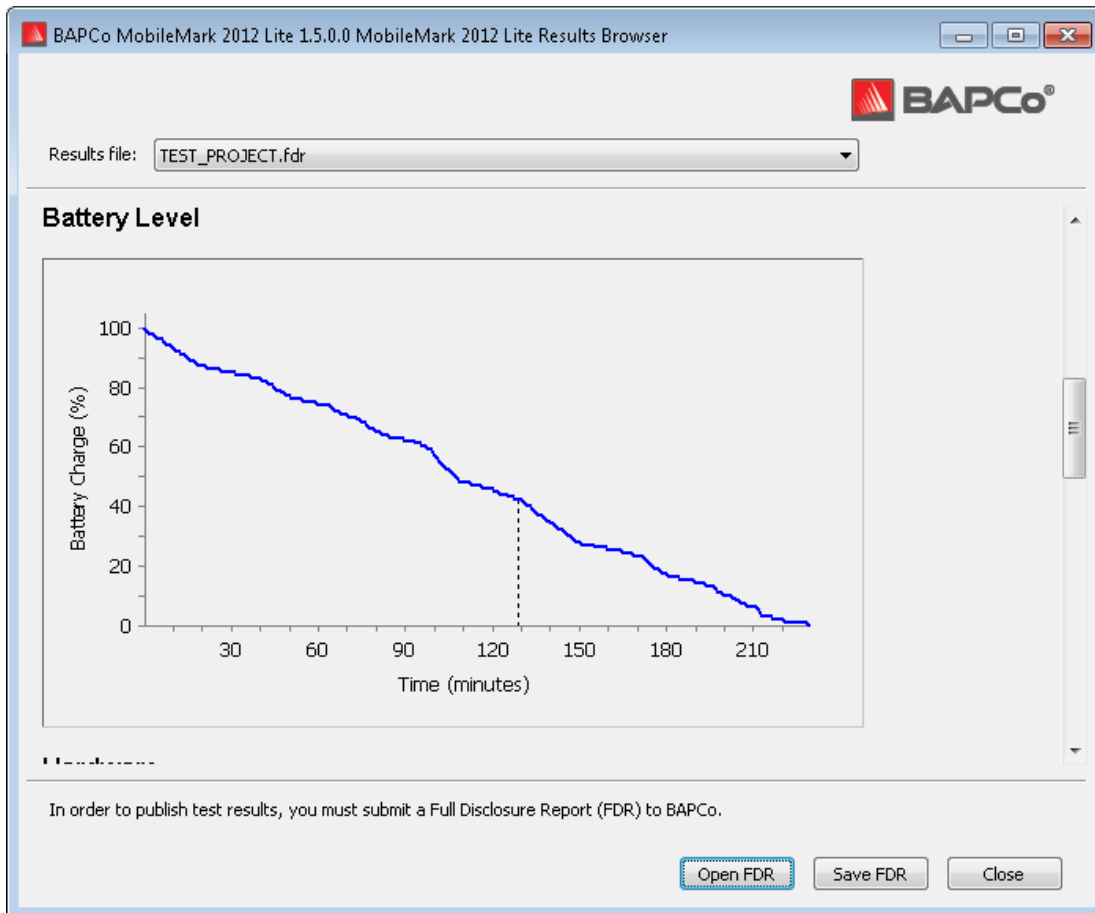
Figure 16: Example of Office Productivity scenario battery chart.
