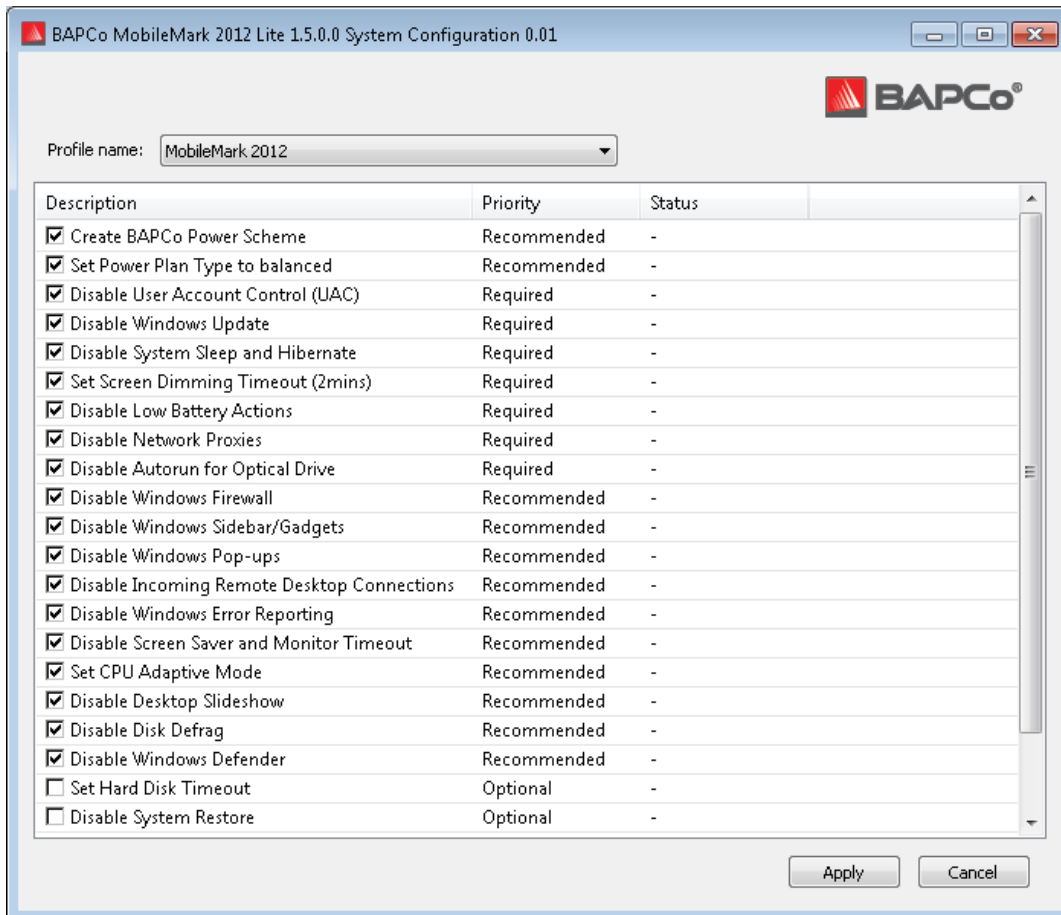
Figure 11: MobileMark 2012 Lite configuration tool, shown with default options selected.
