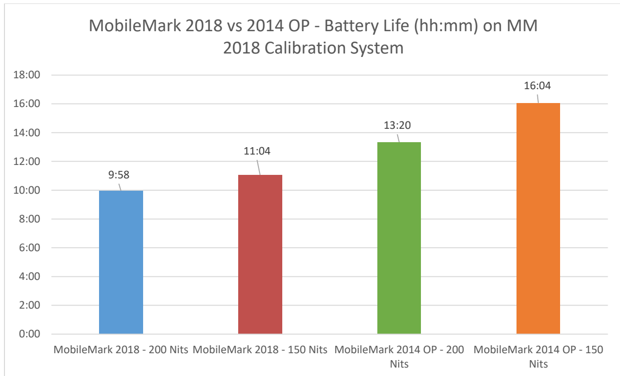
Figure 7: Battery Life of the Calibration System (See Section 2.7 for system details) on MobileMark 2018 with a display brightness of 200 nits, MobileMark 2018 with a display brightness of 150 nits, MobileMark 2014 OP with a display brightness of 200 nits, MobileMark 2014 OP with a display brightness of 150 nits. xi
